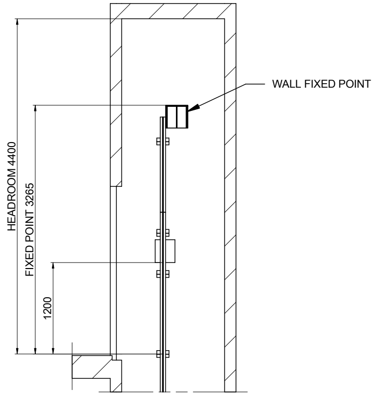
COUNTERWEIGHT OPPOSITE WALL SCALE[*]: 1:50
