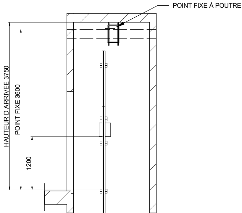
MUR OPPOSE AU CONTREPOIDS ECHELLE[*]: 1:50
